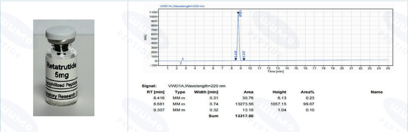
HPLC Chromatogram (Retention Time: 8.681 min)
