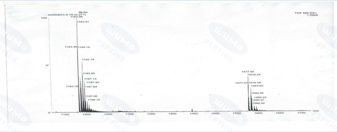
Mass Spectrum (ESI-MS)
