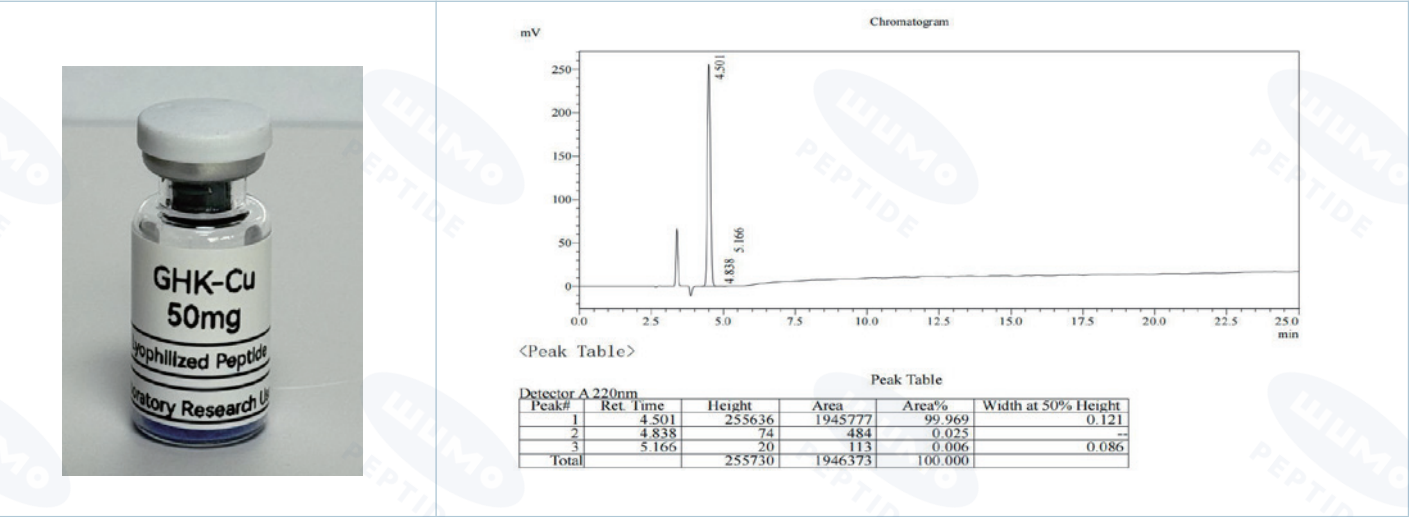
HPLC Chromatogram (Retention Time: 4.501 min)
