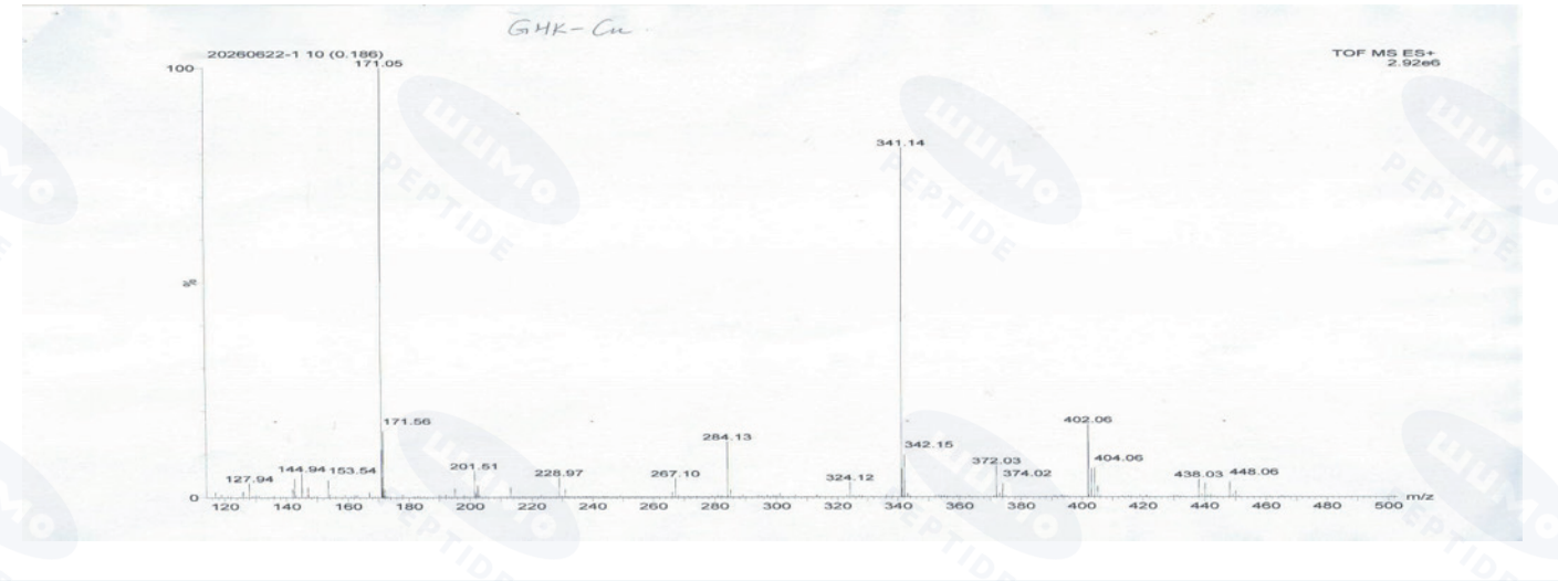
Mass Spectrum (ESI-MS)
