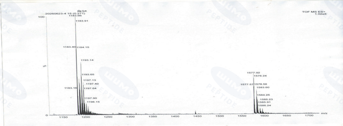
Mass Spectrum (ESI-MS)
